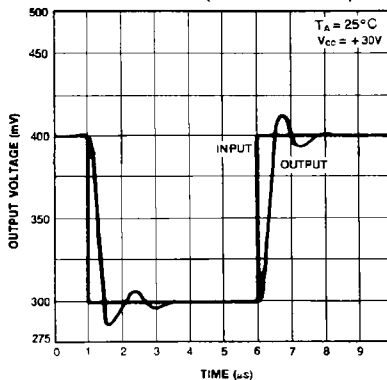
Fig. 8 VOLTAGE FOLLOWER PULSE RESPONSE (SMALL SIGNAL)
