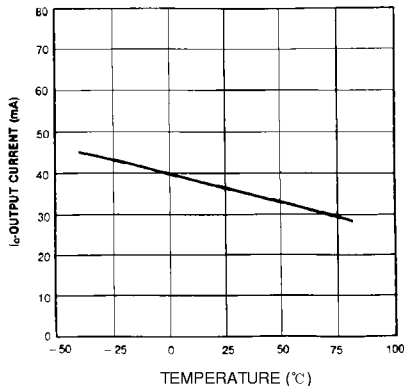
Fig. 12 CURRENT LIMITING
