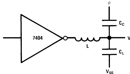
FIGURE 5. Clock Coupling
