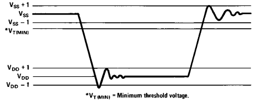
FIGURE 3. Clock Waveform
