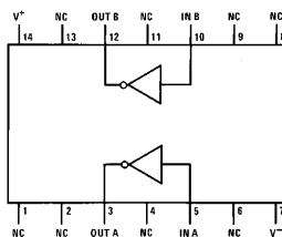
Dual-In-Line Package
