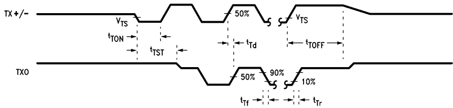
FIGURE 6. Transmitter Timing
