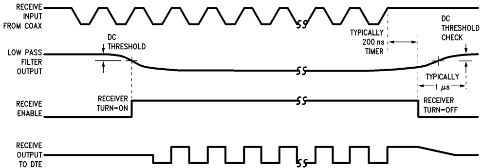
FIGURE 2. Receiver Timing
