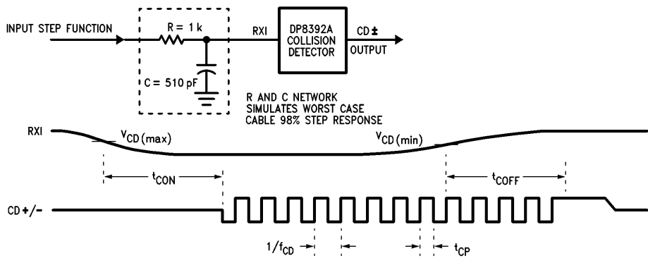
FIGURE 7. Collision Timing
