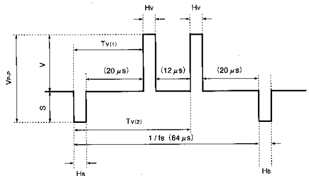
Fig. 2 Output waveform
